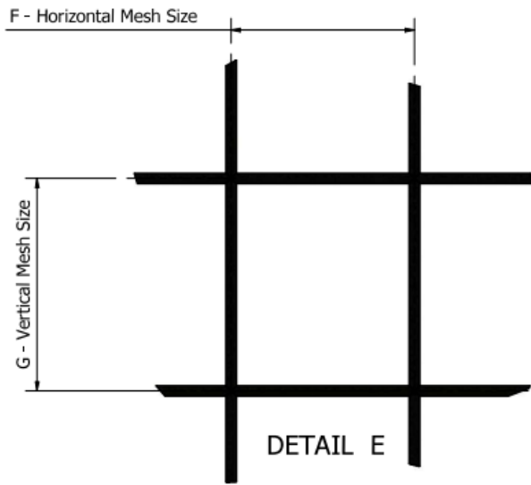
Figure 2 The dimension of the net- a mask.
