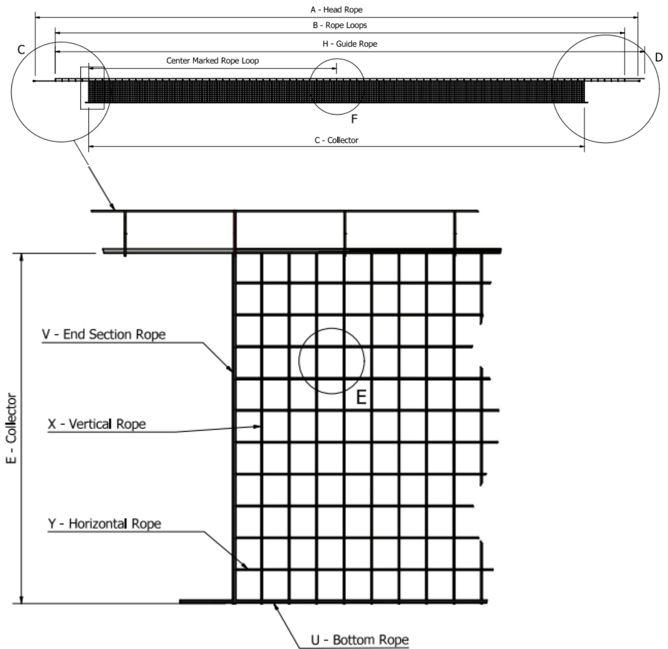
Figure 1 The dimensions of the net - overview
